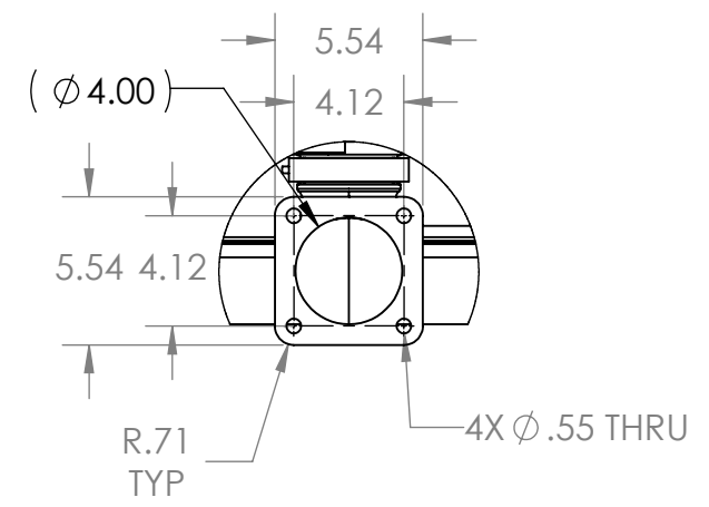
DETAIL A DRY EXHAUST FLANGE SCALE 1 : 8
